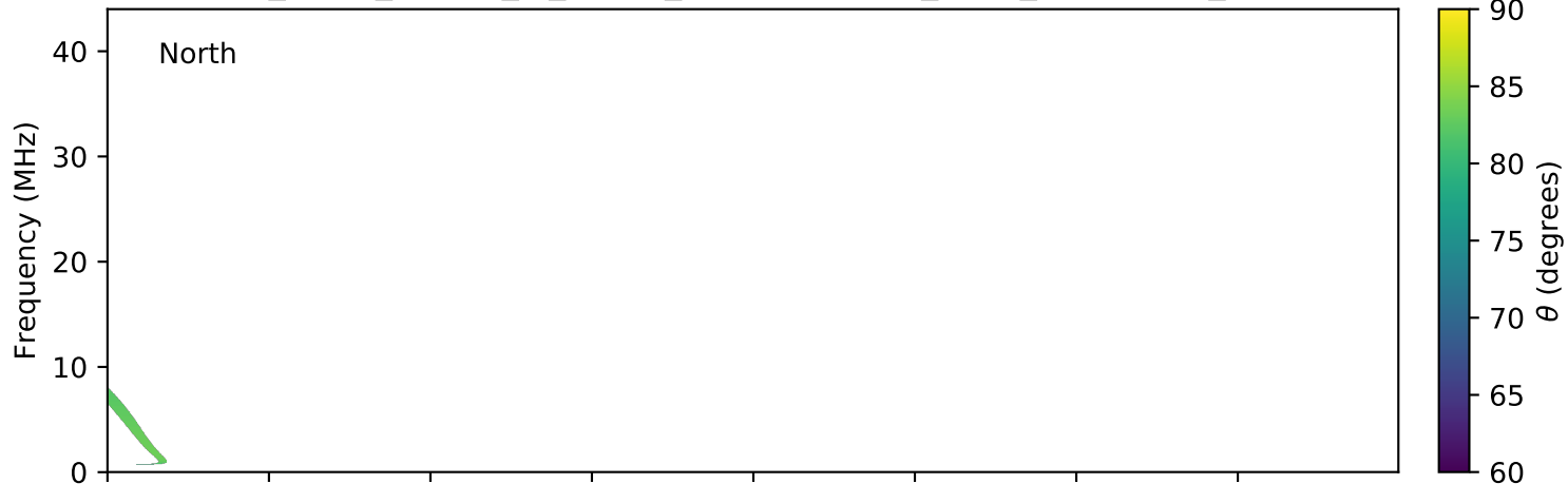
expres_earth_jupiter_io_jrm09_lossc-wid1deg_3kev_20060919_v01.cdf
