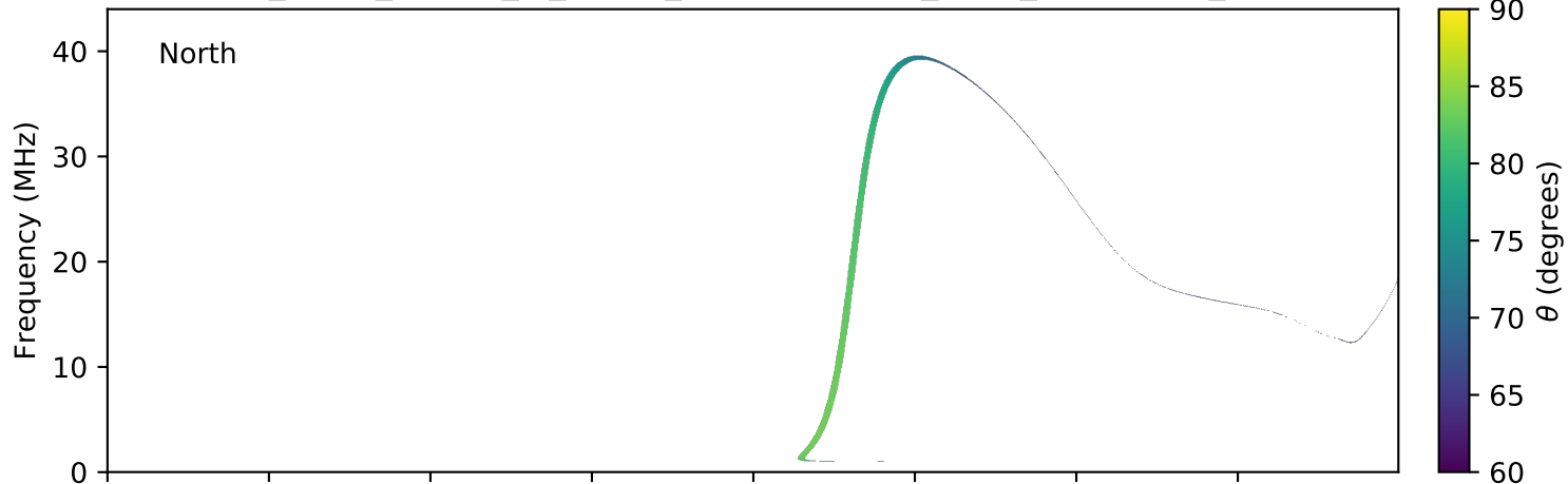
expres_earth_jupiter_io_jrm09_lossc-wid1deg_3kev_20060916_v01.cdf
