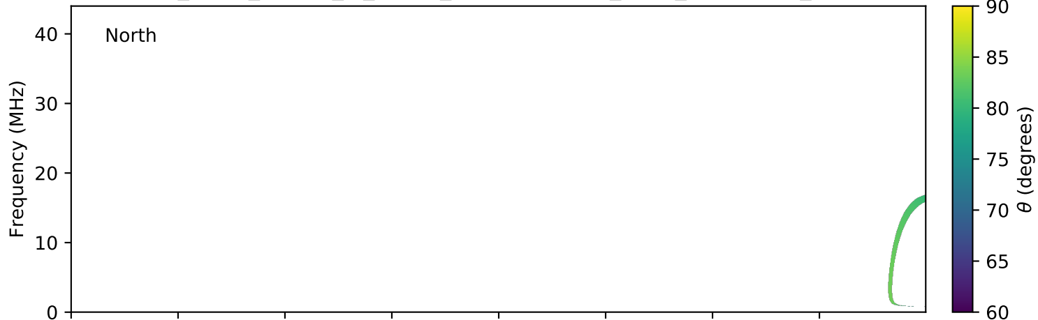
expres_earth_jupiter_io_jrm09_lossc-wid1deg_3kev_20060912_v01.cdf
