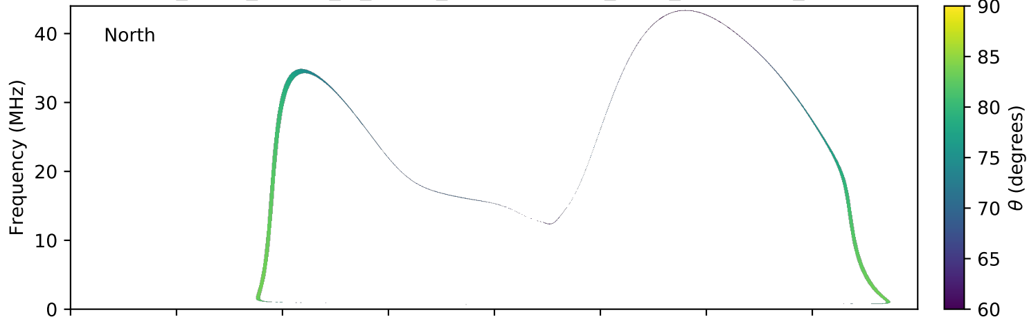
expres_earth_jupiter_io_jrm09_lossc-wid1deg_3kev_20060911_v01.cdf
