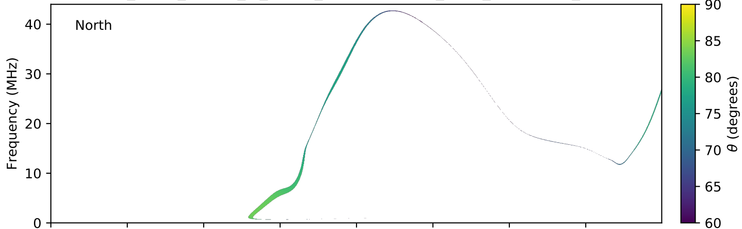
expres_earth_jupiter_io_jrm09_lossc-wid1deg_3kev_20060902_v01.cdf
