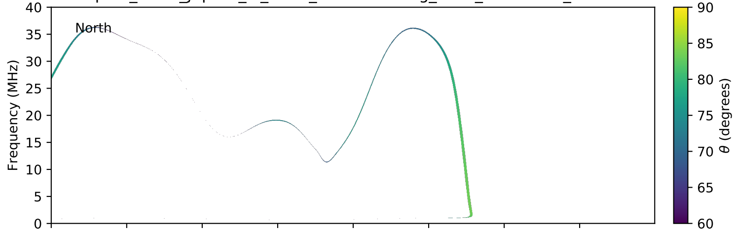
expres_earth_jupiter_io_isaac_lossc-wid1deg_3kev_20060929_v01.cdf
