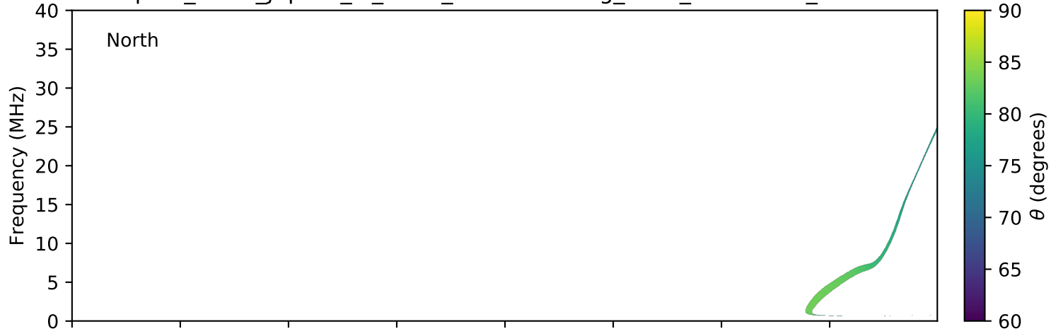
expres_earth_jupiter_io_isaac_lossc-wid1deg_3kev_20060928_v01.cdf
