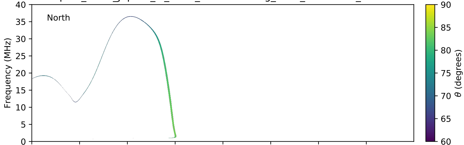
expres_earth_jupiter_io_isaac_lossc-wid1deg_3kev_20060924_v01.cdf
