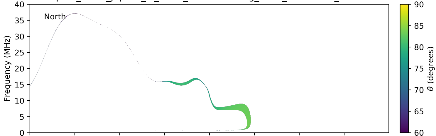
expres_earth_jupiter_io_isaac_lossc-wid1deg_3kev_20060922_v01.cdf
