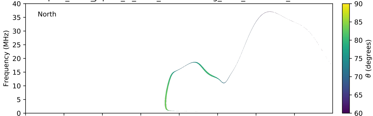
expres_earth_jupiter_io_isaac_lossc-wid1deg_3kev_20060916_v01.cdf
