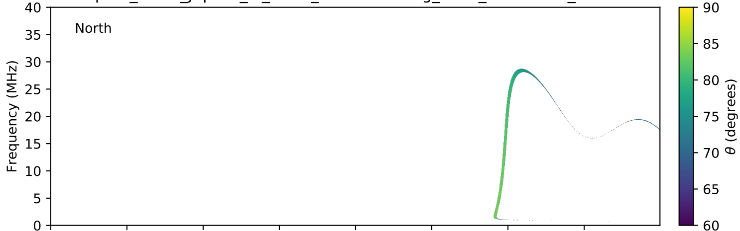
expres_earth_jupiter_io_isaac_lossc-wid1deg_3kev_20060914_v01.cdf
