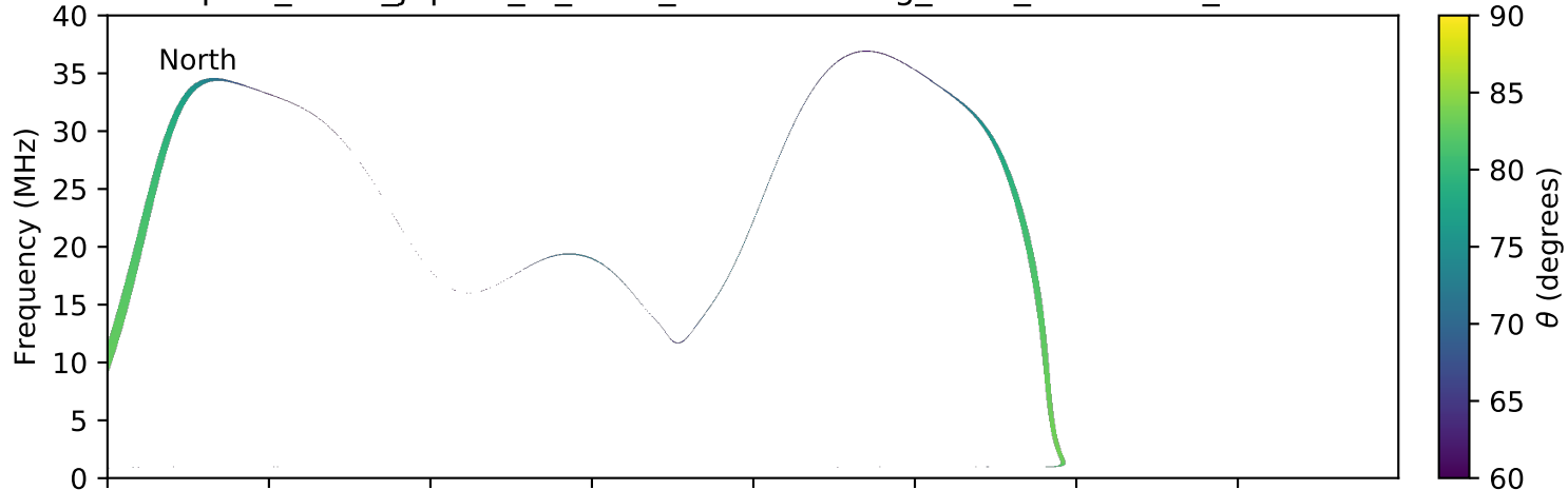
expres_earth_jupiter_io_isaac_lossc-wid1deg_3kev_20060913_v01.cdf
