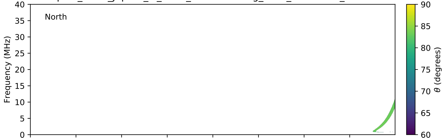
expres_earth_jupiter_io_isaac_lossc-wid1deg_3kev_20060912_v01.cdf
