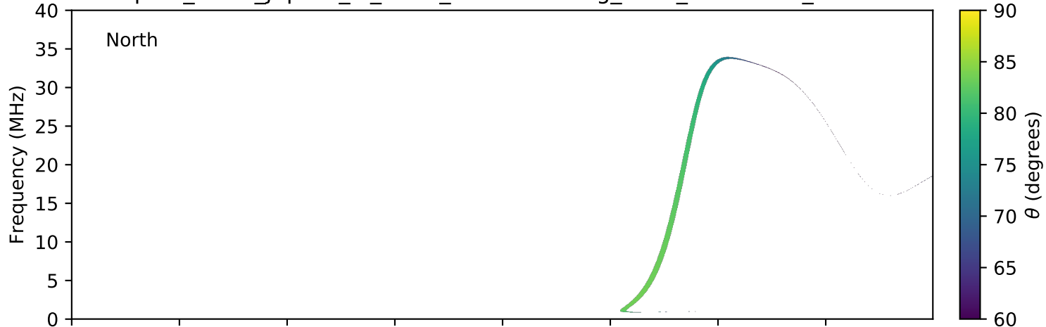
expres_earth_jupiter_io_isaac_lossc-wid1deg_3kev_20060907_v01.cdf
