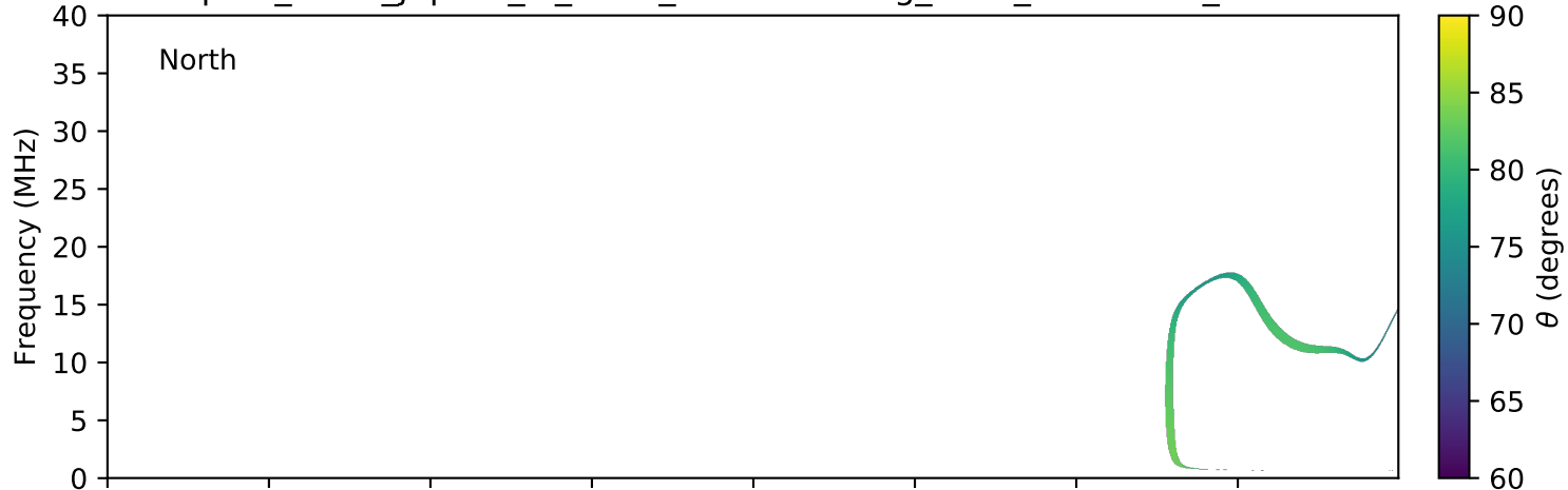
expres_earth_jupiter_io_isaac_lossc-wid1deg_3kev_20060905_v01.cdf
