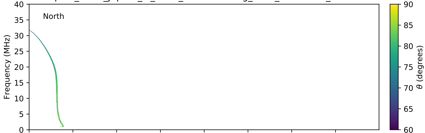
expres_earth_jupiter_io_isaac_lossc-wid1deg_3kev_20060903_v01.cdf
