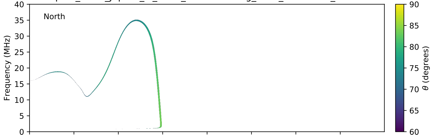
expres_earth_jupiter_io_isaac_lossc-wid1deg_3kev_20060901_v01.cdf
