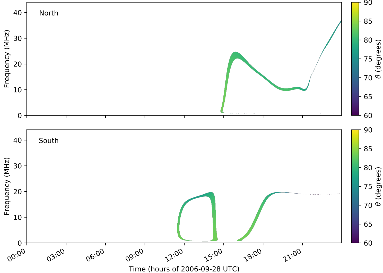
expres_earth_jupiter_europa_jrm09_lossc-wid1deg_3kev_20060928_v01.cdf
