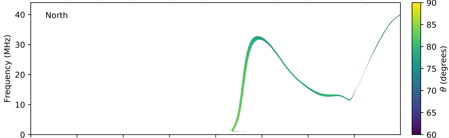
expres_earth_jupiter_europa_jrm09_lossc-wid1deg_3kev_20060921_v01.cdf
