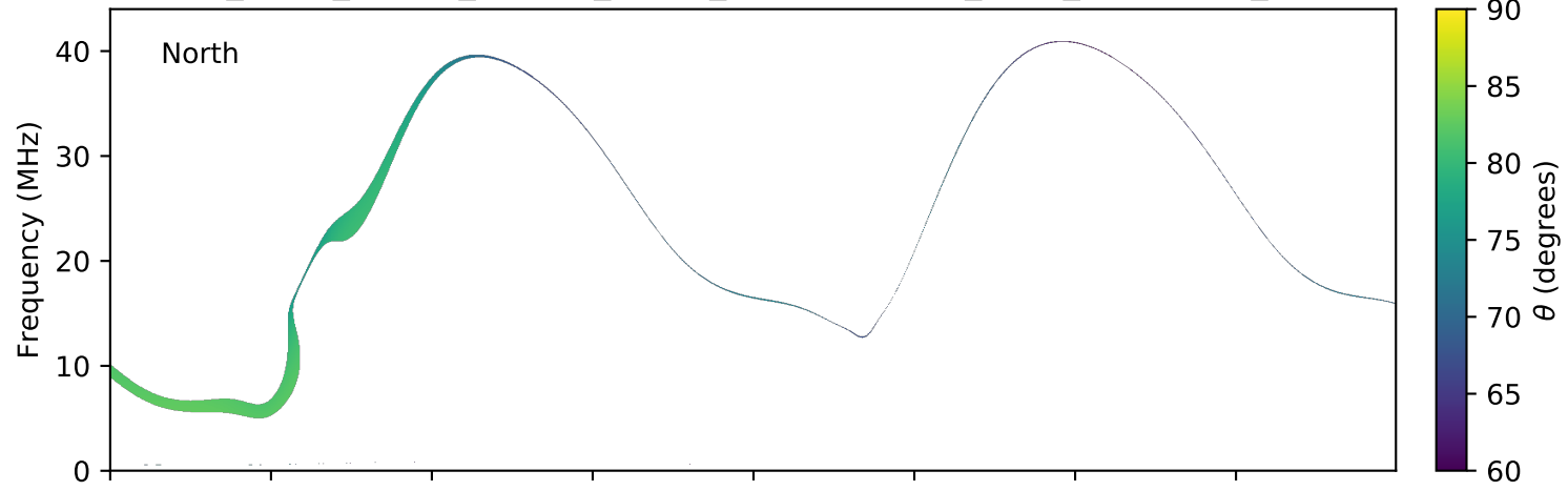
expres_earth_jupiter_europa_jrm09_lossc-wid1deg_3kev_20060918_v01.cdf
