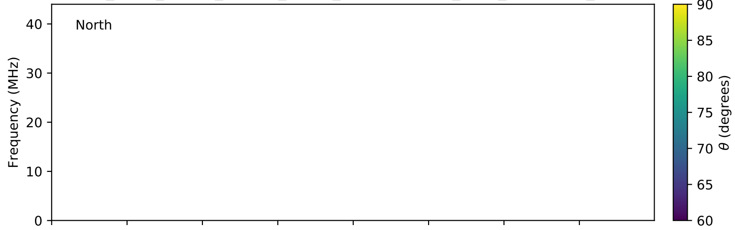
expres_earth_jupiter_europa_jrm09_lossc-wid1deg_3kev_20060909_v01.cdf
