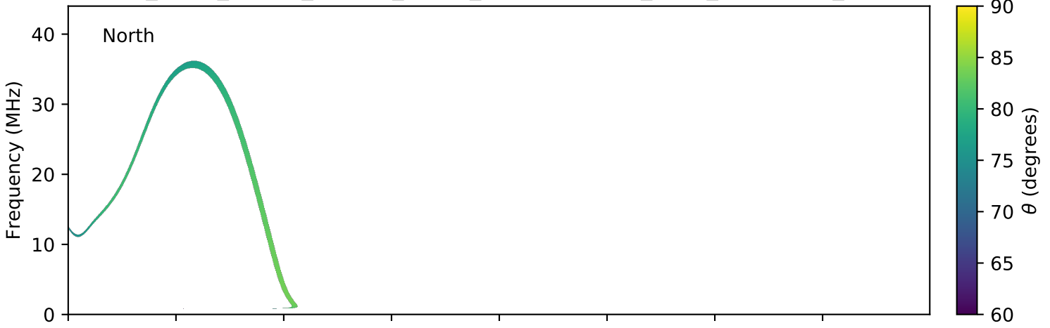
expres_earth_jupiter_europa_jrm09_lossc-wid1deg_3kev_20060905_v01.cdf
