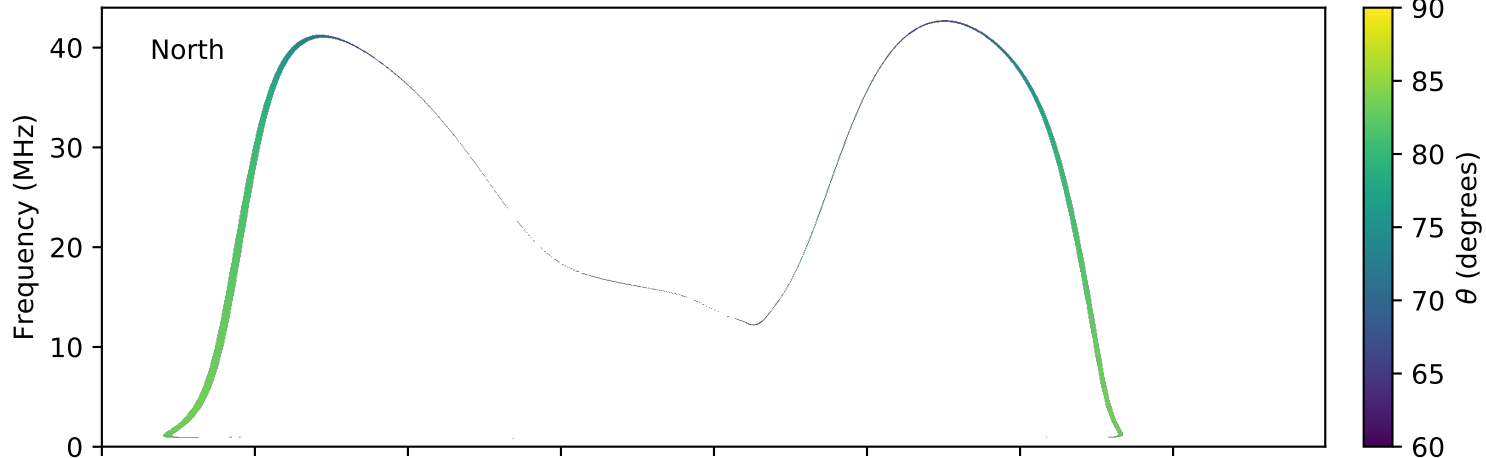
expres_earth_jupiter_io_jrm09_lossc-wid1deg_3kev_20060828_v01.cdf
