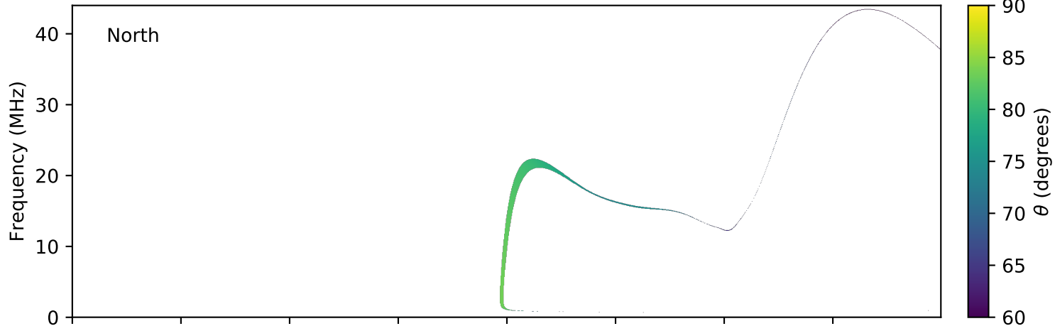
expres_earth_jupiter_io_jrm09_lossc-wid1deg_3kev_20060824_v01.cdf
