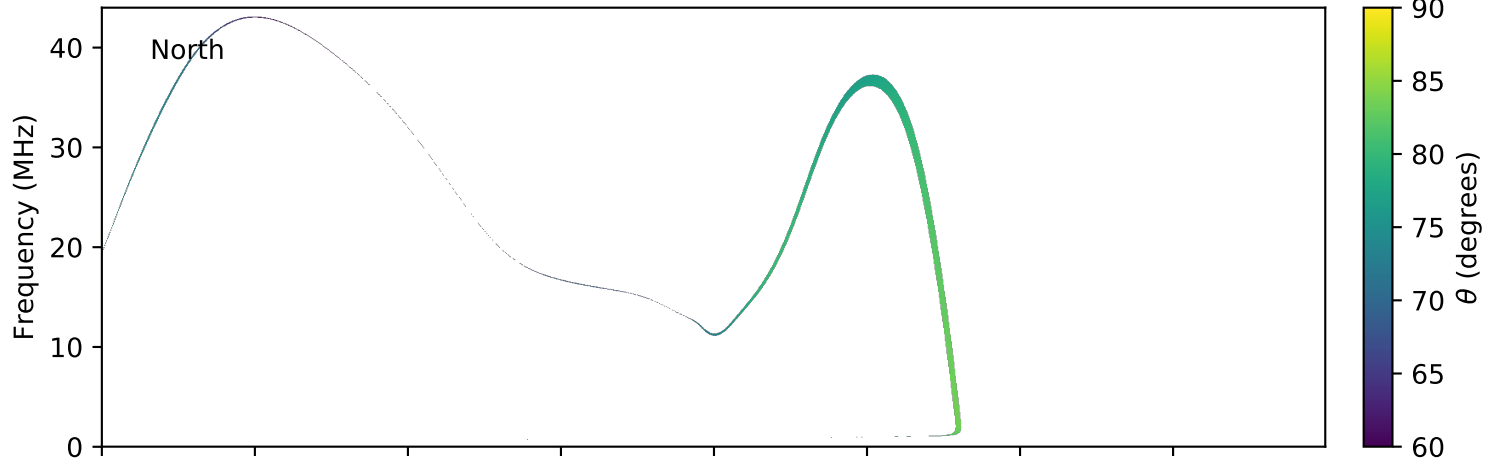
expres_earth_jupiter_io_jrm09_lossc-wid1deg_3kev_20060814_v01.cdf
