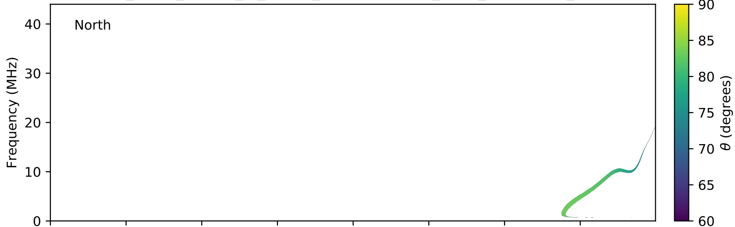
expres_earth_jupiter_io_jrm09_lossc-wid1deg_3kev_20060813_v01.cdf
