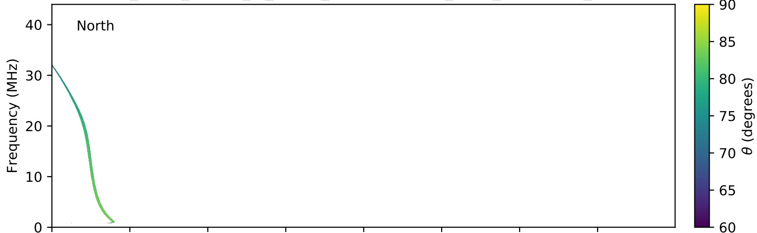
expres_earth_jupiter_io_jrm09_lossc-wid1deg_3kev_20060811_v01.cdf
