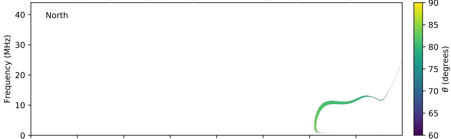
expres_earth_jupiter_io_jrm09_lossc-wid1deg_3kev_20060806_v01.cdf
