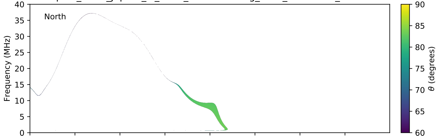
expres_earth_jupiter_io_isaac_lossc-wid1deg_3kev_20060830_v01.cdf
