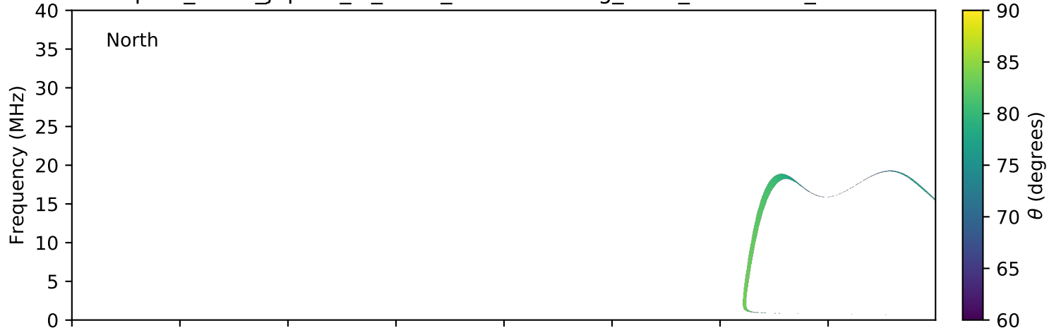
expres_earth_jupiter_io_isaac_lossc-wid1deg_3kev_20060829_v01.cdf
