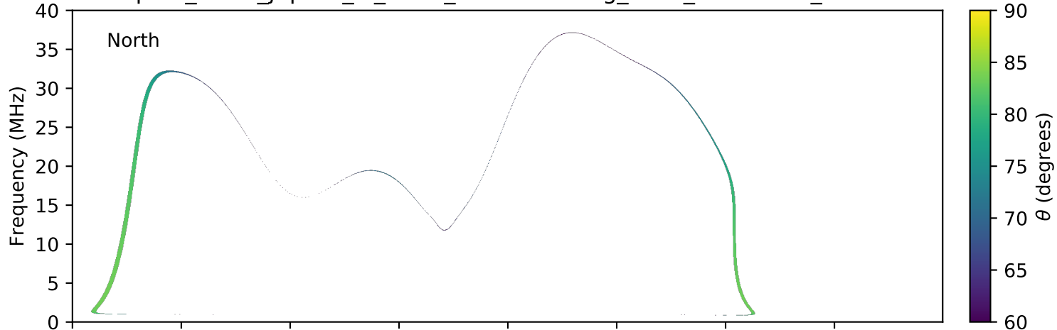
expres_earth_jupiter_io_isaac_lossc-wid1deg_3kev_20060828_v01.cdf
