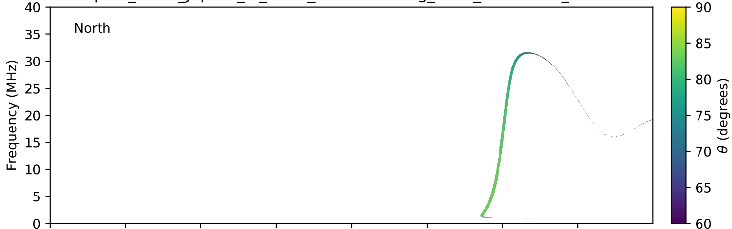
expres_earth_jupiter_io_isaac_lossc-wid1deg_3kev_20060822_v01.cdf
