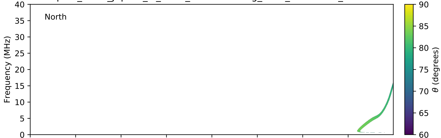
expres_earth_jupiter_io_isaac_lossc-wid1deg_3kev_20060820_v01.cdf
