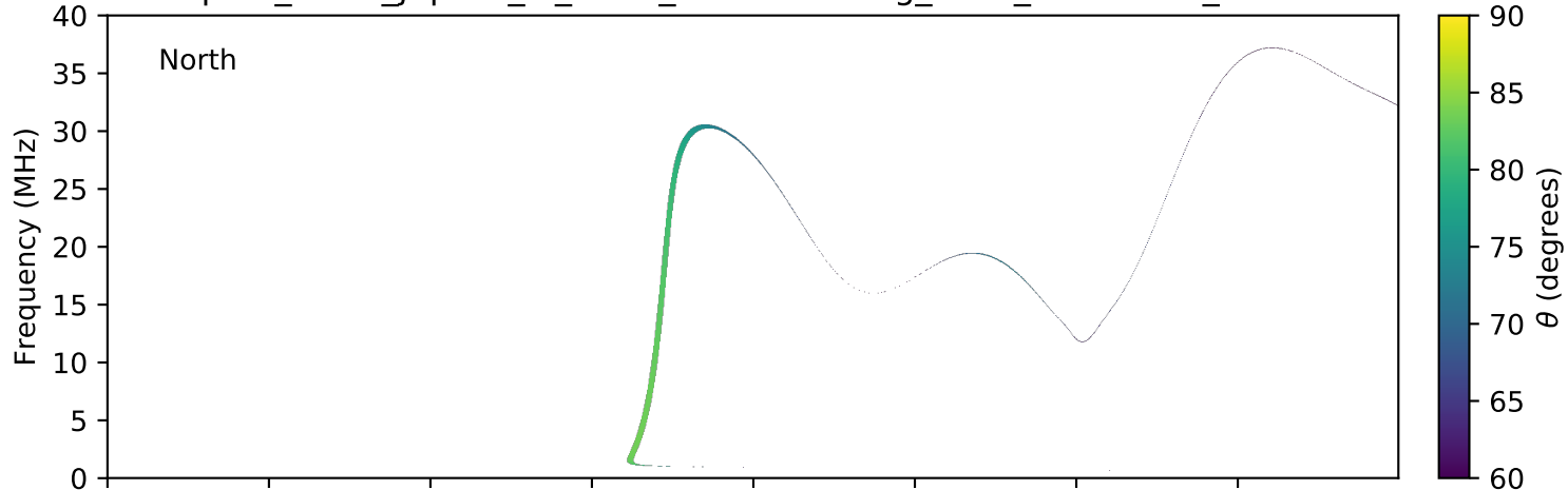
expres_earth_jupiter_io_isaac_lossc-wid1deg_3kev_20060817_v01.cdf
