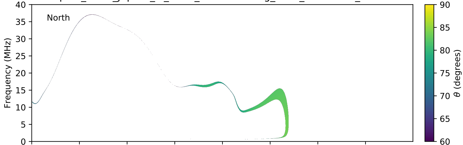
expres_earth_jupiter_io_isaac_lossc-wid1deg_3kev_20060814_v01.cdf
