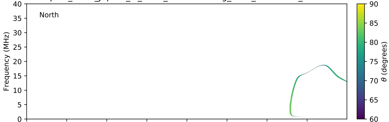
expres_earth_jupiter_io_isaac_lossc-wid1deg_3kev_20060813_v01.cdf
