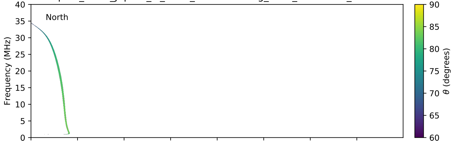
expres_earth_jupiter_io_isaac_lossc-wid1deg_3kev_20060811_v01.cdf
