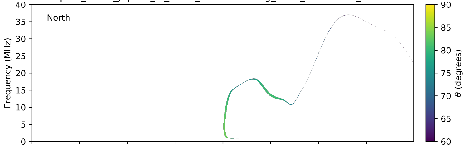
expres_earth_jupiter_io_isaac_lossc-wid1deg_3kev_20060808_v01.cdf
