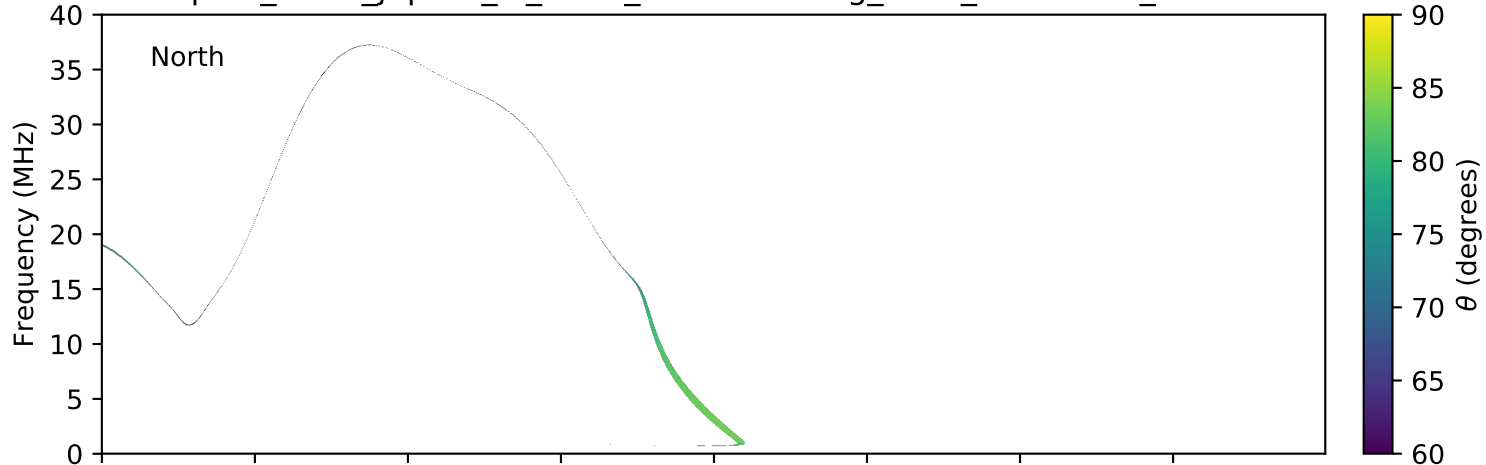
expres_earth_jupiter_io_isaac_lossc-wid1deg_3kev_20060807_v01.cdf
