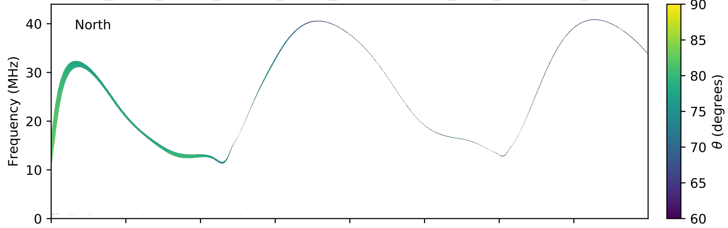
expres_earth_jupiter_europa_jrm09_lossc-wid1deg_3kev_20060817_v01.cdf
