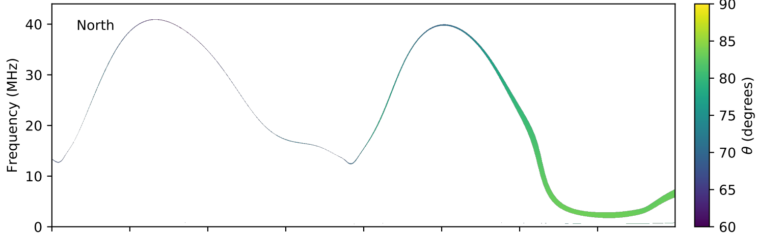
expres_earth_jupiter_europa_jrm09_lossc-wid1deg_3kev_20060814_v01.cdf
