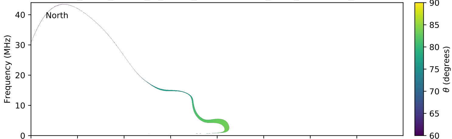
expres_earth_jupiter_io_jrm09_lossc-wid1deg_3kev_20060731_v01.cdf
