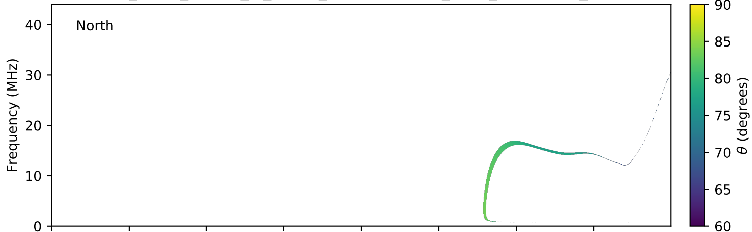
expres_earth_jupiter_io_jrm09_lossc-wid1deg_3kev_20060730_v01.cdf
