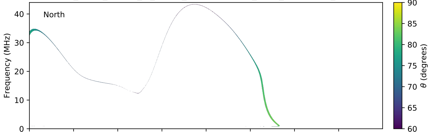
expres_earth_jupiter_io_jrm09_lossc-wid1deg_3kev_20060729_v01.cdf
