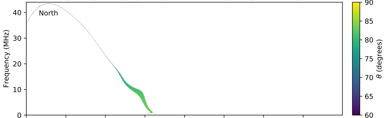
expres_earth_jupiter_io_jrm09_lossc-wid1deg_3kev_20060724_v01.cdf
