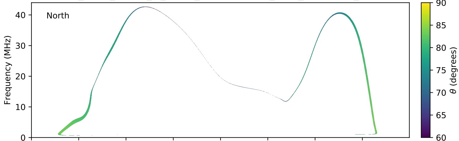
expres_earth_jupiter_io_jrm09_lossc-wid1deg_3kev_20060720_v01.cdf
