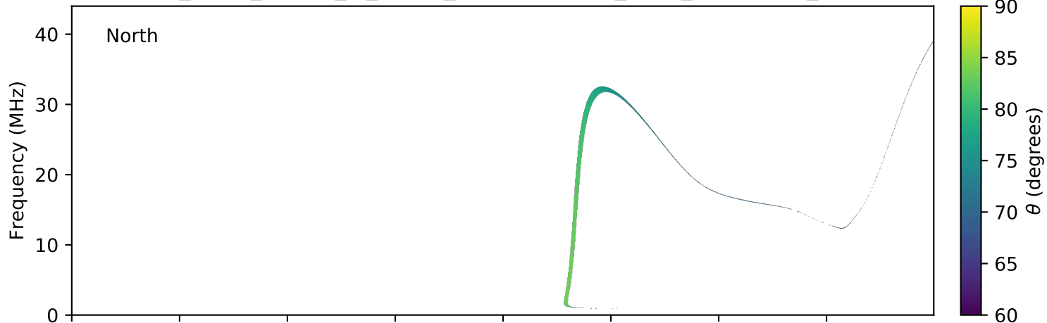
expres_earth_jupiter_io_jrm09_lossc-wid1deg_3kev_20060716_v01.cdf
