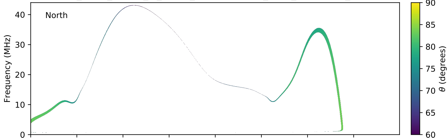
expres_earth_jupiter_io_jrm09_lossc-wid1deg_3kev_20060713_v01.cdf
