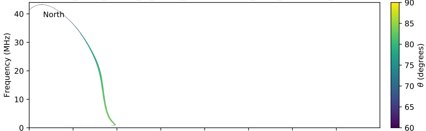
expres_earth_jupiter_io_jrm09_lossc-wid1deg_3kev_20060710_v01.cdf
