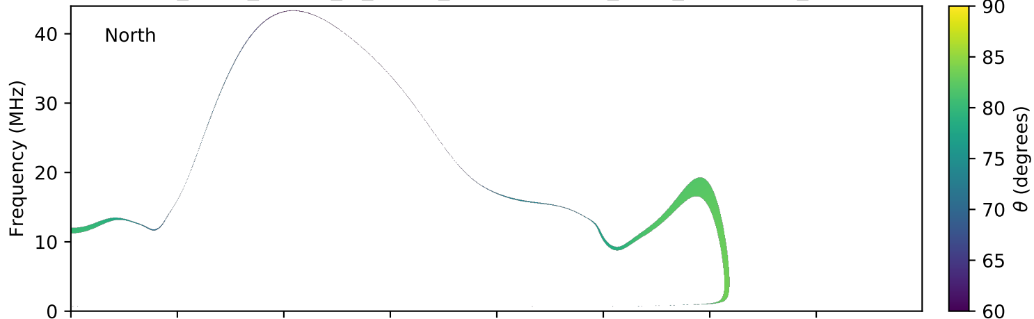
expres_earth_jupiter_io_jrm09_lossc-wid1deg_3kev_20060706_v01.cdf
